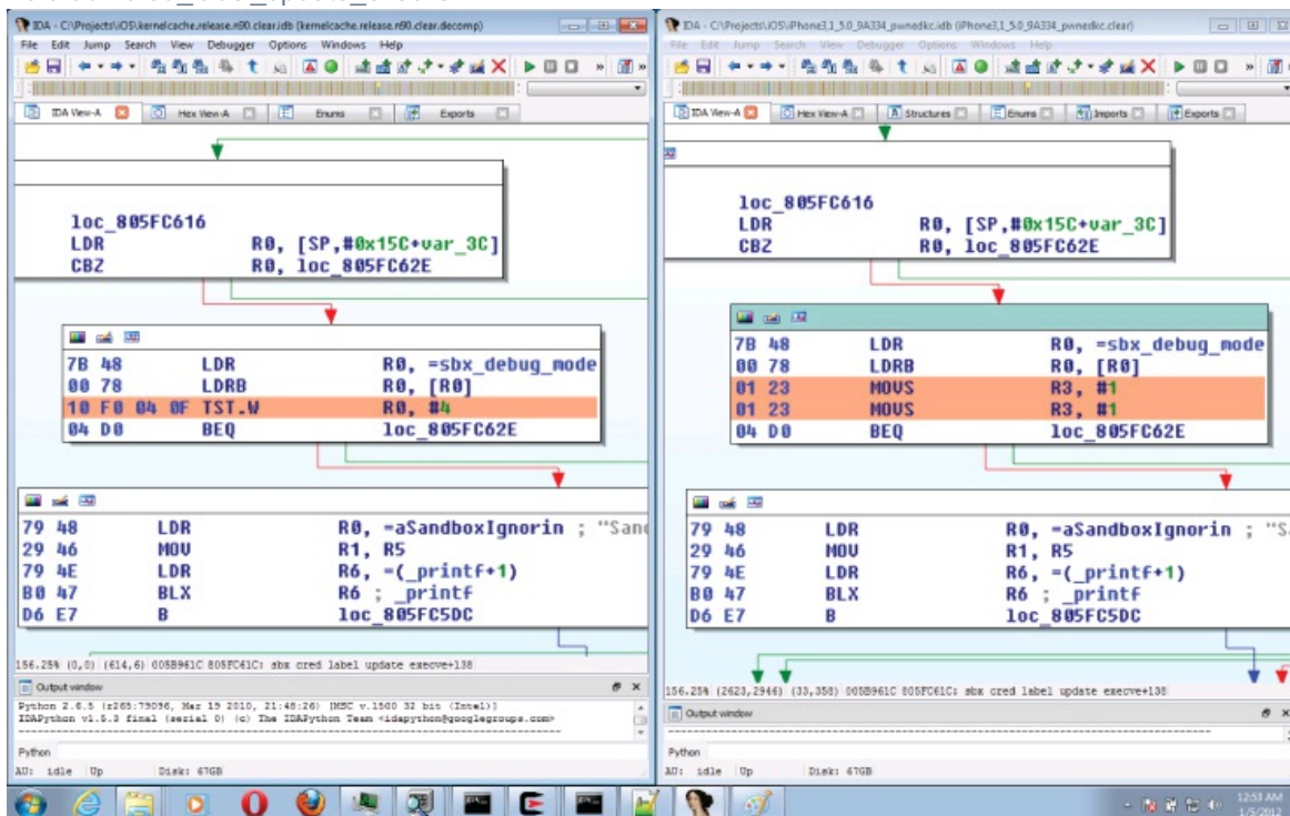
Figure 5.3 redsn0w 0.9.9b7 cred_label_update_execve
