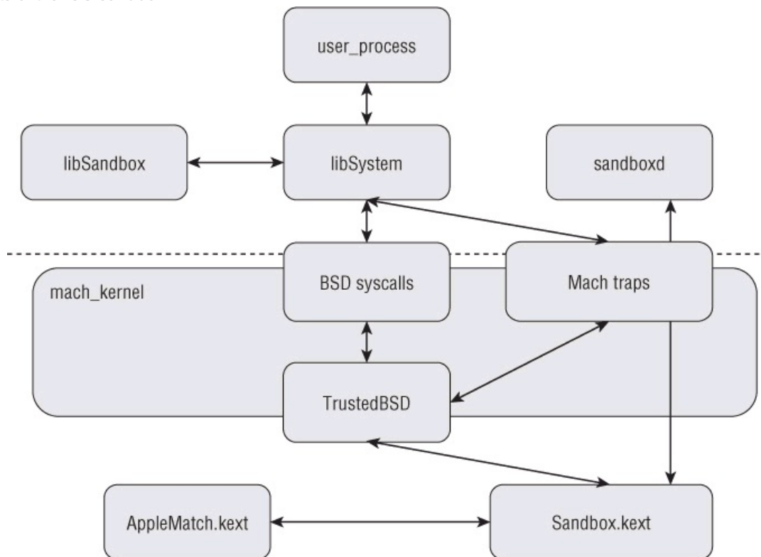
Figure 5.1 Components of the iOS sandbox
