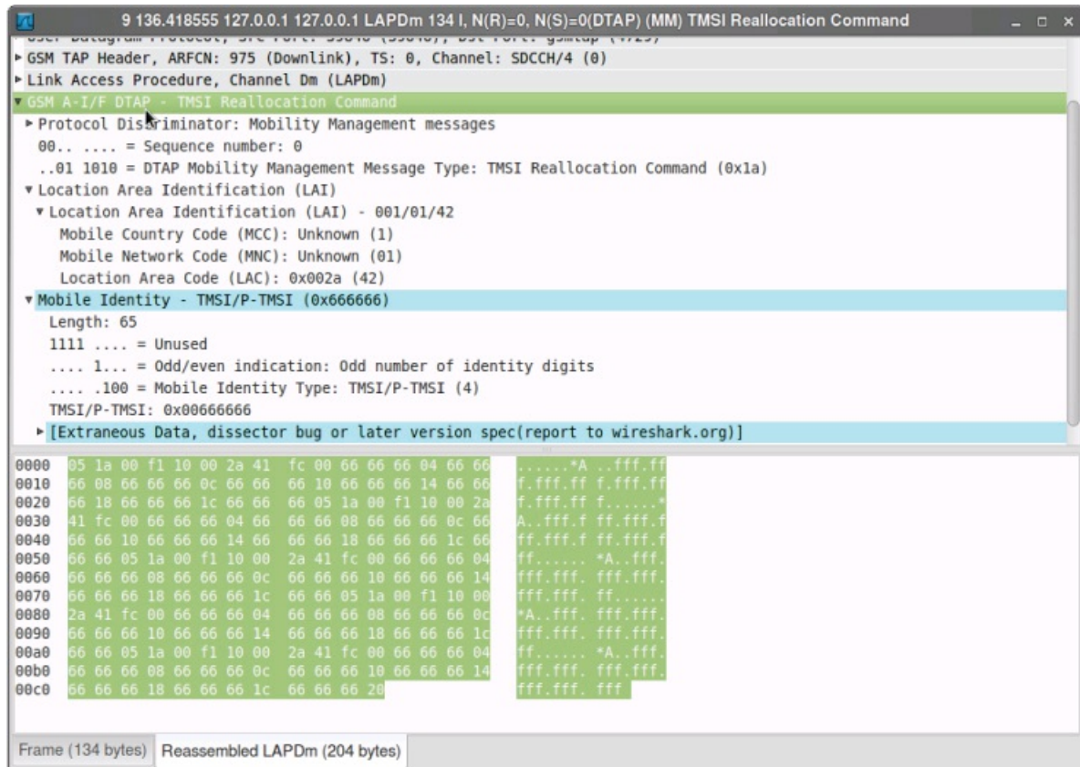
Figure 11.3 Malicious TMSI REALLOCATION COMMAND dissected with Wireshark
