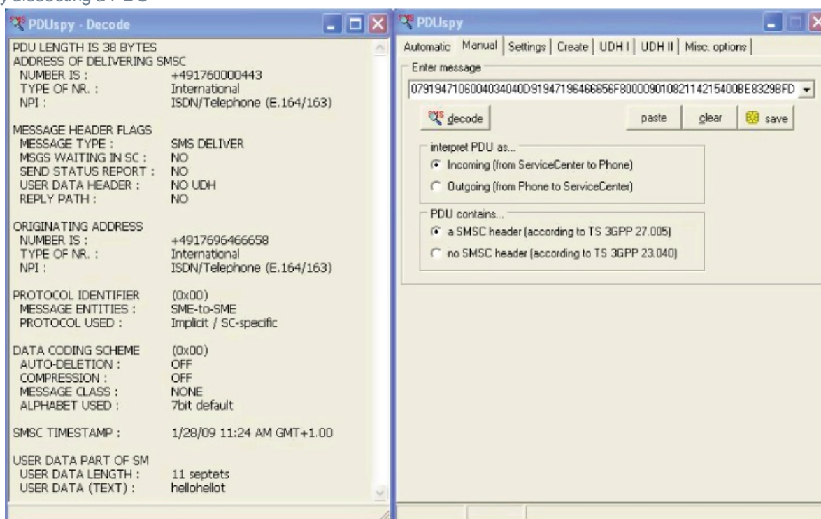
Figure 6.7 PDUspy dissecting a PDU
