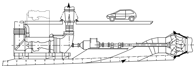
FIGURE 31.16 Rolls-Royce Marine Spey machinery arrangement for a waterjet-powered fast ferry
