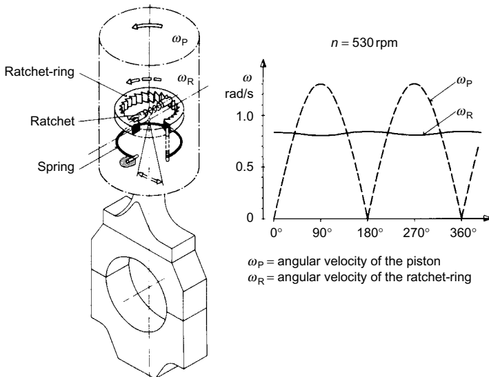
FIGURE 26.4 Drive principle of rotating piston
