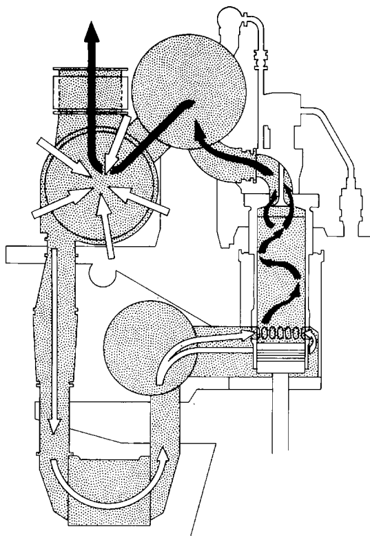
FIGURE I.14 Burmeister & Wain uniflow-scavenging system
