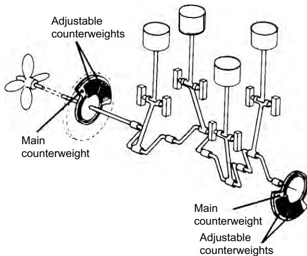
FIGURE 1.12 Four-cylinder MAN B&W 500–980 mm bore MC engines are fitted with adjustable counterweights
