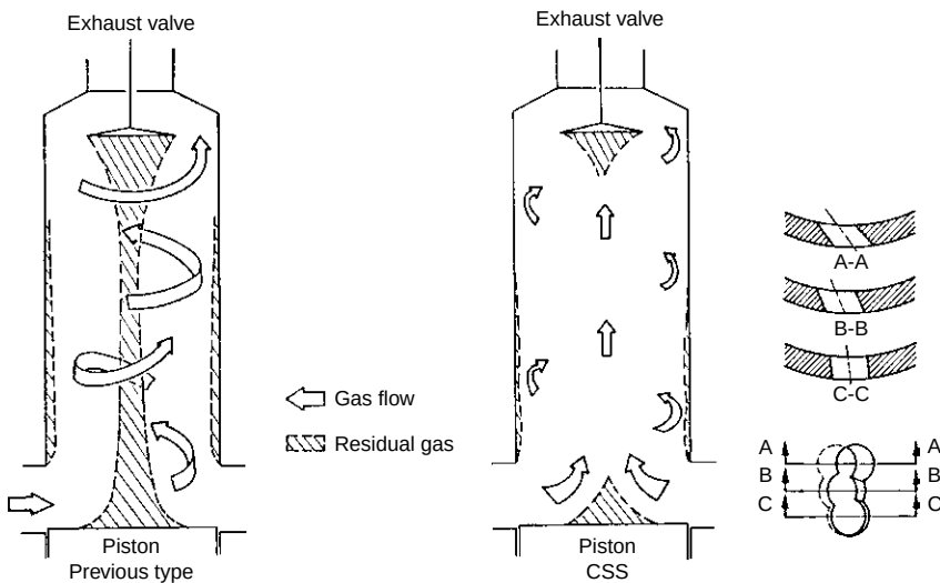
FIGURE 11.12 Comparison of gas flow in cylinder with original UE engine scavenging and with controlled swirl scavenging (CSS)
