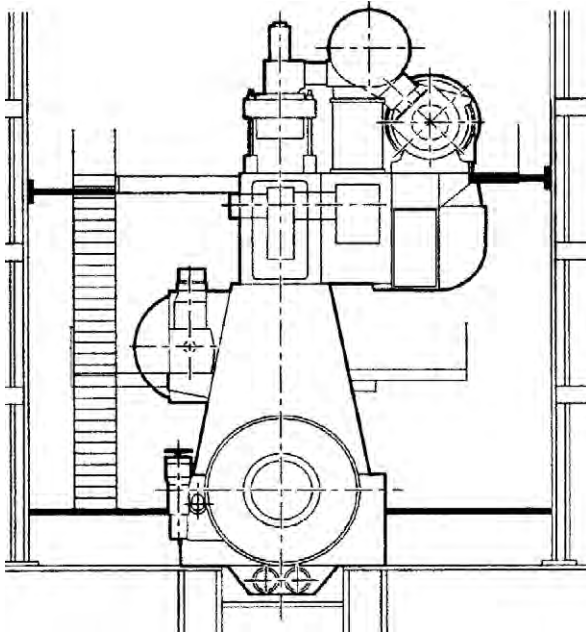
FIGURE 1.20 Typical attachment points for transverse stays of Wärtsilä RTA low-speed engine
