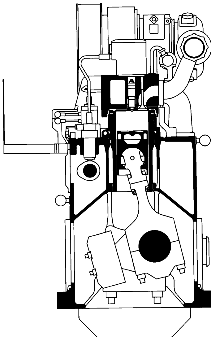
FIGURE 26.16 Cross-section of ZA50S engine
