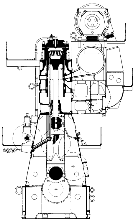
FIGURE 12.39 Cross-section of 900-mm bore Sulzer RLB90 engine
