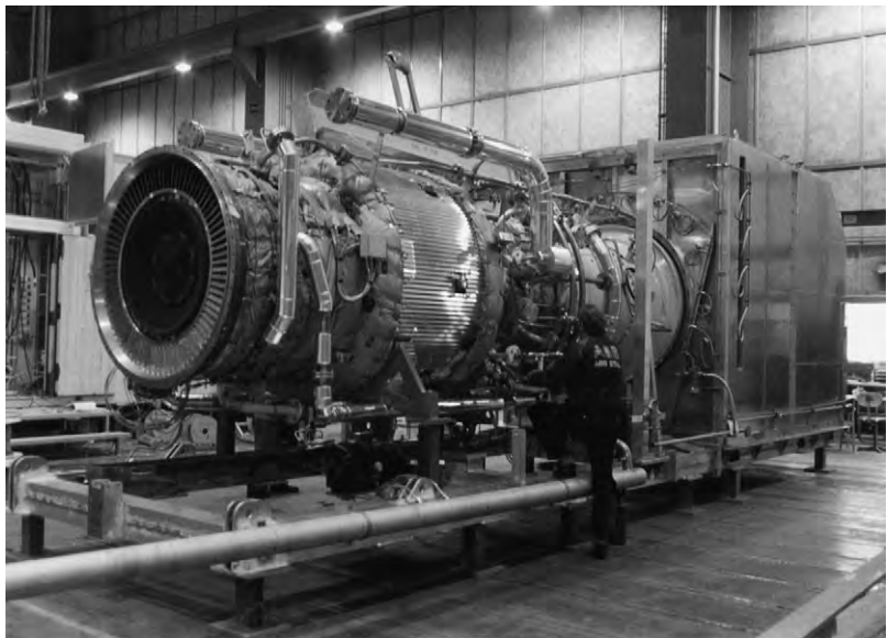
FIGURE 31.11 One of two 17 000 kW ABB Stal GT35 (now designated Siemens SGT-500) gas turbines supplied to drive the waterjets of a Stena HSS 900-class fast ferry
