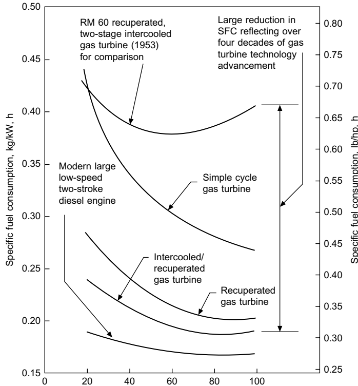
FIGURE 31.5 Comparison of sfc curves against load for various gas turbine cycles and a low-speed two-stroke diesel engine
