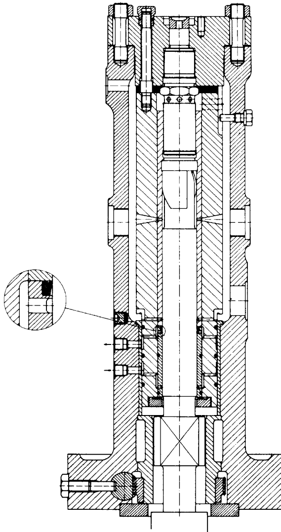
FIGURE 13.9 Fuel pump
