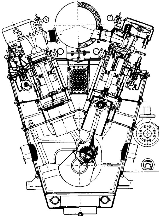
FIGURE 28.30 Cross-section through Bolnes VDNL 150/600 two-stroke engine
