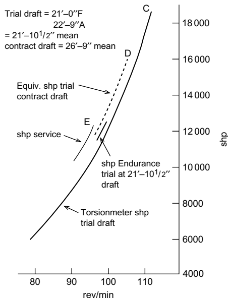
FIGURE 5.4 Propulsion data
