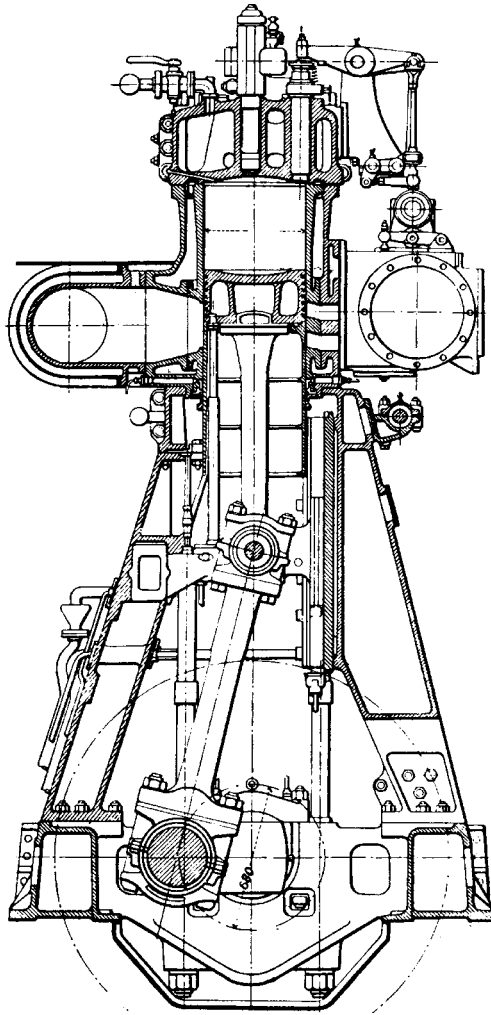
FIGURE I.4 Twin Sulzer 4S47 type cross-flow scavenged crosshead engines served the Monte Penedo , the first large oceangoing vessel powered by two-stroke engines (1912). Four long tie-rods secured each cylinder head directly to the bedplate, holding the whole cast iron engine structure in compression
