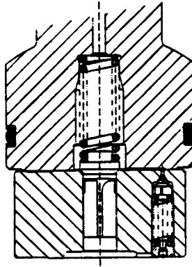
FIGURE 8.15 Typical pressure unloading delivery valve design (Delphi Bryce)
