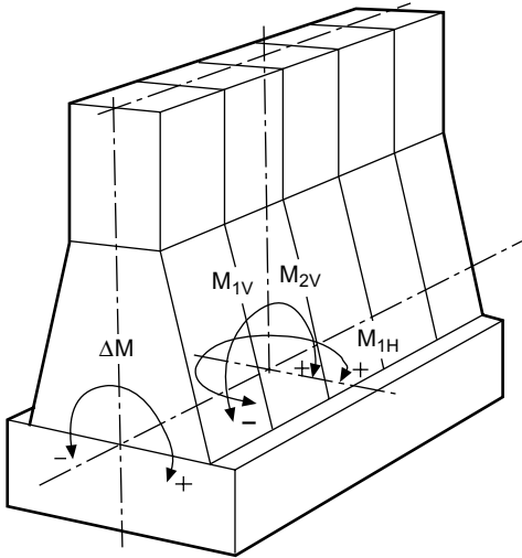
FIGURE 1.11b Free couples of mass forces and the torque variation about the centre lines of the engine and crankshaft (Wärtsilä): M_{1V} is the first-order couple having a vertical component. M_{1H} is the first-order couple having a horizontal component. M_{2V} is the second-order couple having a vertical component. \Delta M is the reaction to variations in the nominal torque. Reduction of the first-order couples is achieved by counterweights installed at both ends of the crankshaft
