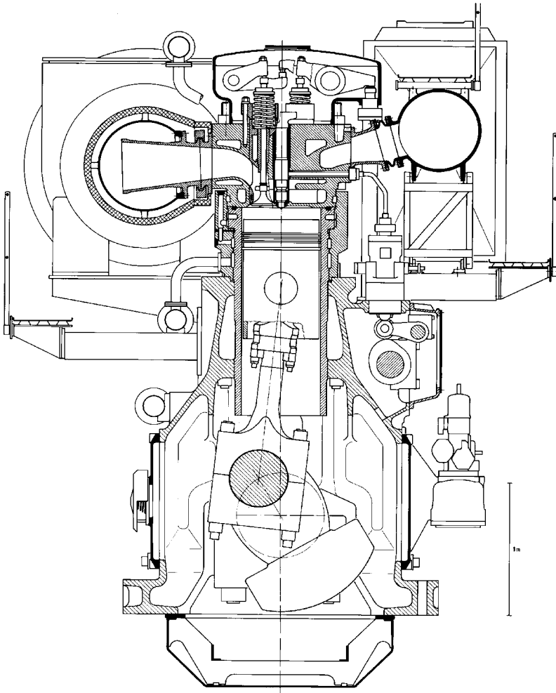
FIGURE 22.3 MAN L58/64 design
