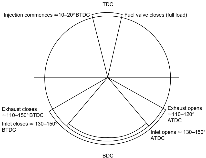
FIGURE 1.6 Two-stroke cycle
