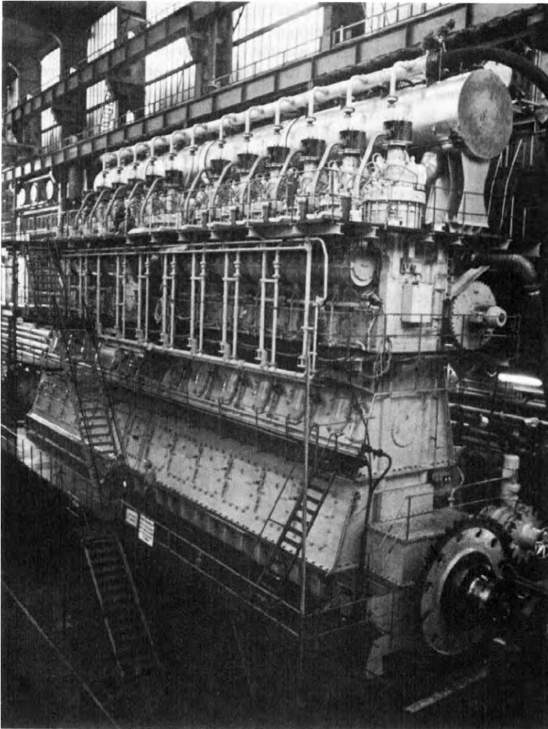
FIGURE 13.12 A 12-cylinder L90GFA engine developing 34 800 kW at 97 rev/min
