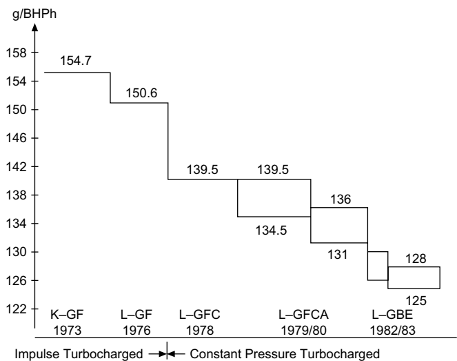
FIGURE I.13 Advances in specific fuel consumption by Burmeister & Wain uniflow-scavenged two-stroke engine designs (900 mm bore models)
