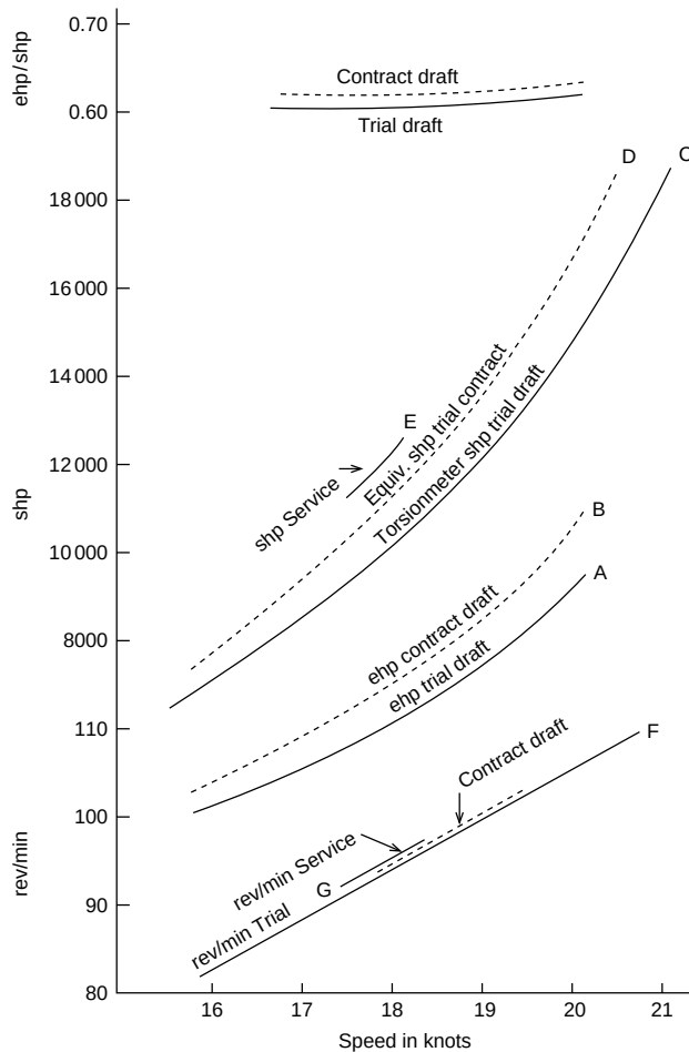
FIGURE 5.3 Propulsion data
