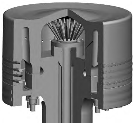
FIGURE 10.45 A spray cooling insert secures a comfortably low piston temperature for the Mark 9-rated large bore engines
