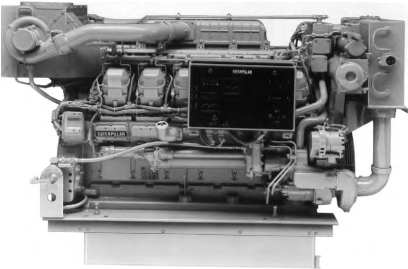
FIGURE 30.3 Caterpillar 3512B engine with ECS
