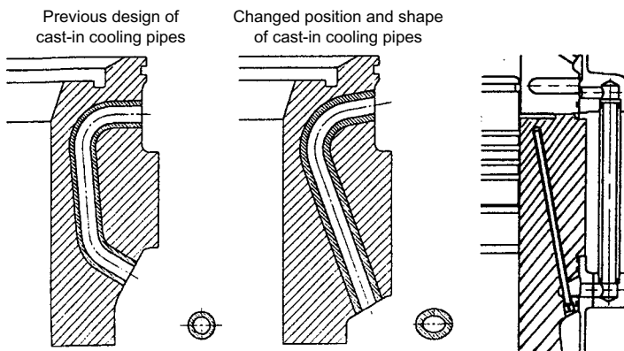
FIGURE 10.20 MC engine cylinder liner modifications. A current bore-cooled standard is shown ( right )
