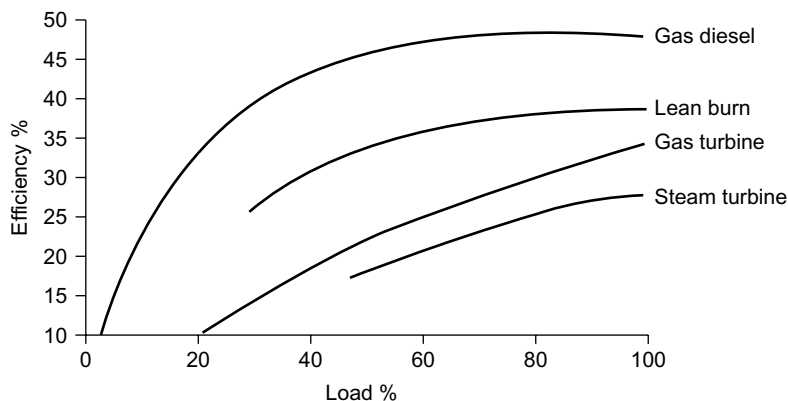
FIGURE 2.1 Thermal efficiency of diesel and GD engines as a function of load (Wärtsilä)
