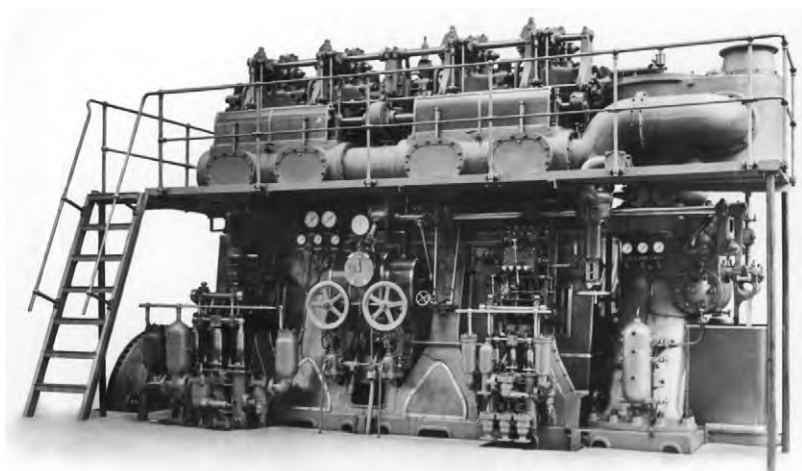
FIGURE I.5 One of the two Sulzer 4S47 engines installed in the Monte Penedo (1912)
