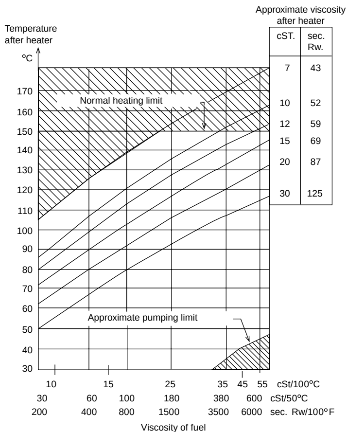
FIGURE 4.8 Fuel oil heating chart (MAN Diesel)
