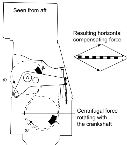
FIGURE 1.13 First-order moment compensator (MAN Diesel)
