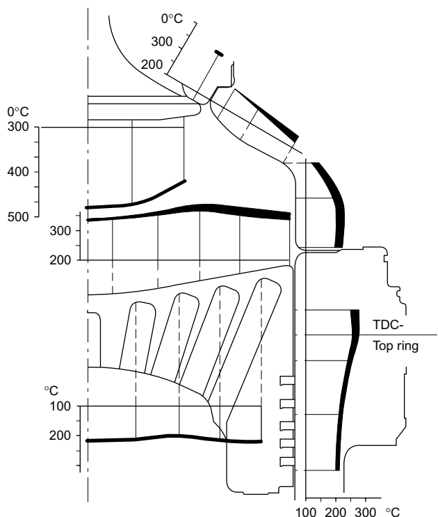
FIGURE 12.23 Surface temperatures measured on the combustion chamber components of the RTA84T-B engine at full load R1 rating. The thickness of the lines represents the circumferential variation in temperature
