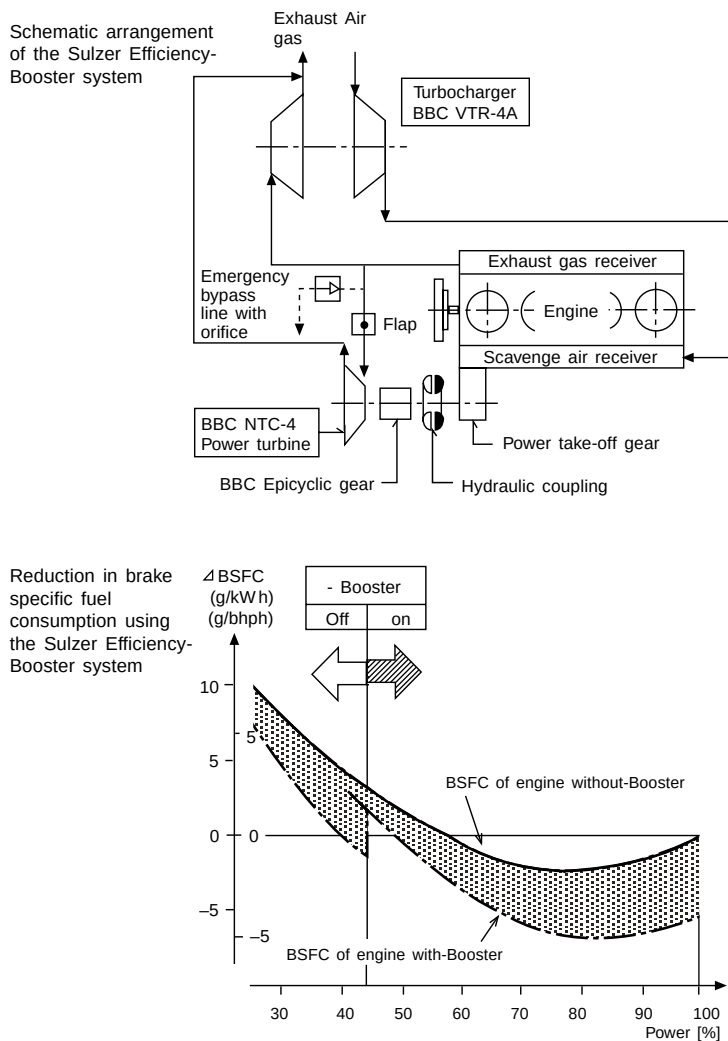
FIGURE 7.31 Sulzer efficiency booster system layout and performance
