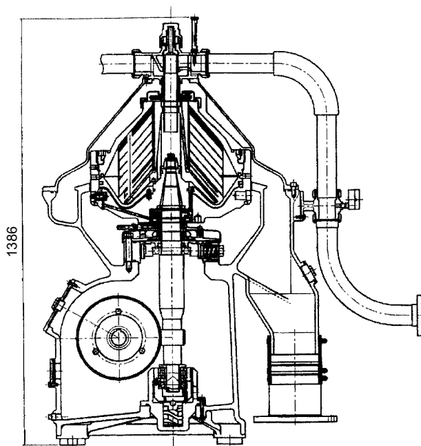
FIGURE 4.6 Mitsubishi Selfjector SJ-FH design centrifugal separator
