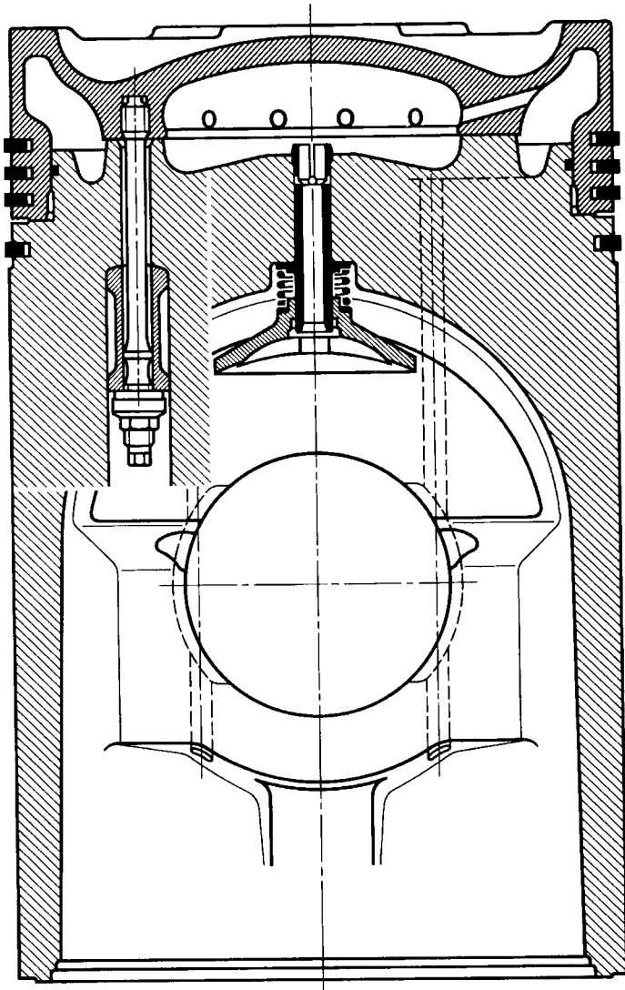
FIGURE 22.11 L58/64 engine composite piston
