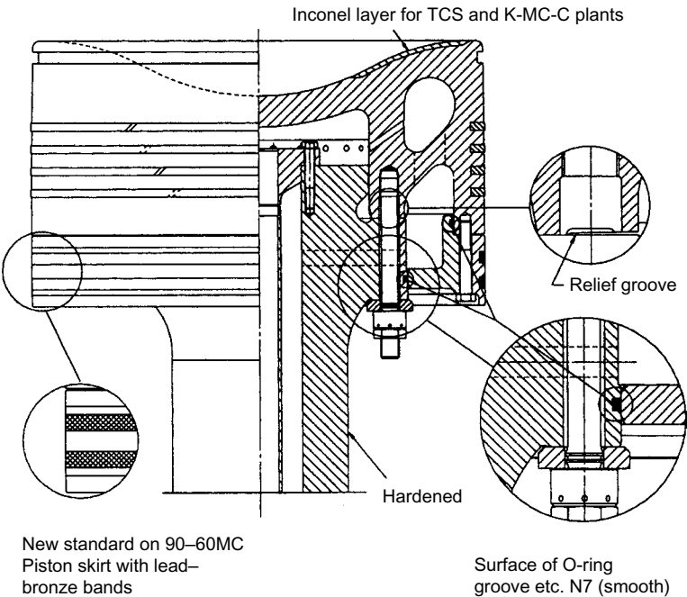
FIGURE 10.6 Piston assembly
