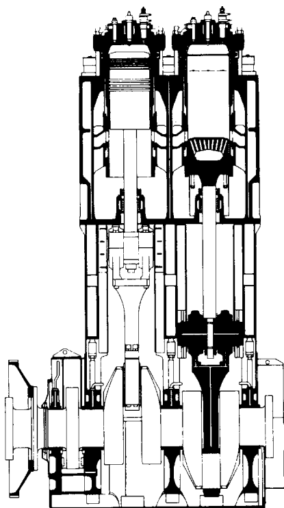
FIGURE 12.40 Longitudinal section of RLB90 engine
