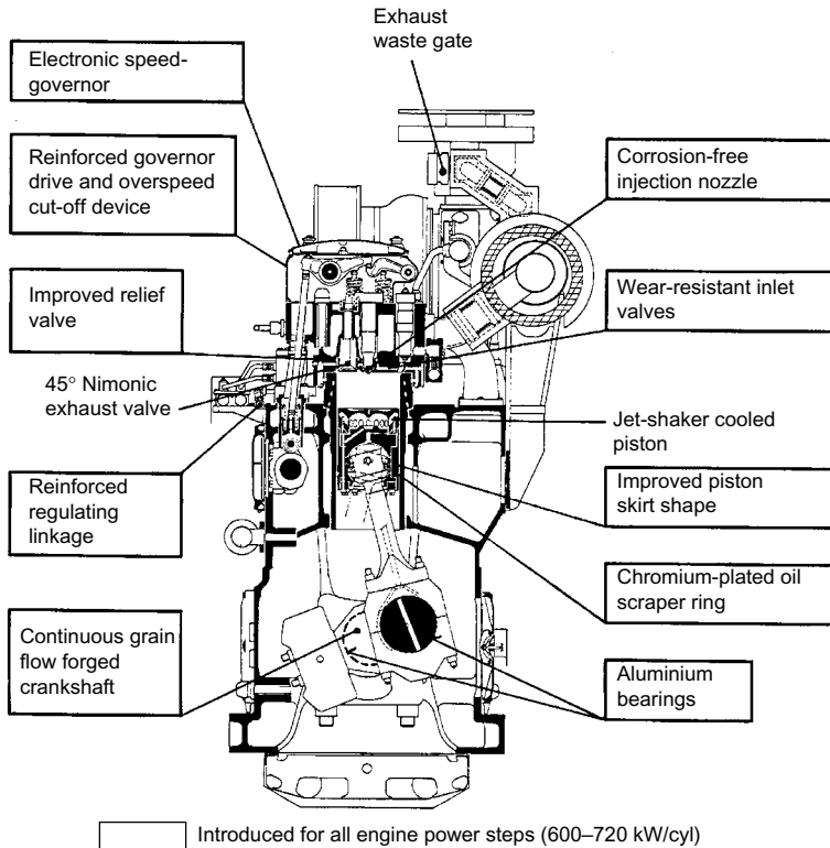
FIGURE 26.3 Main modifications for uprated ZA40S engines
