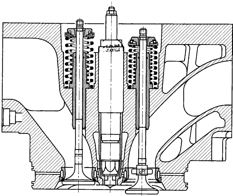
FIGURE 22.22 L32/40 cylinder head
