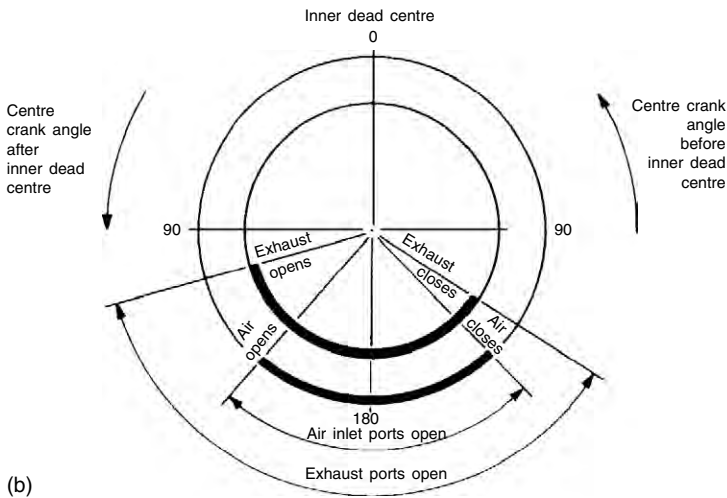
FIGURE 14.4b Port timing diagram for Doxford 76J4C engine
