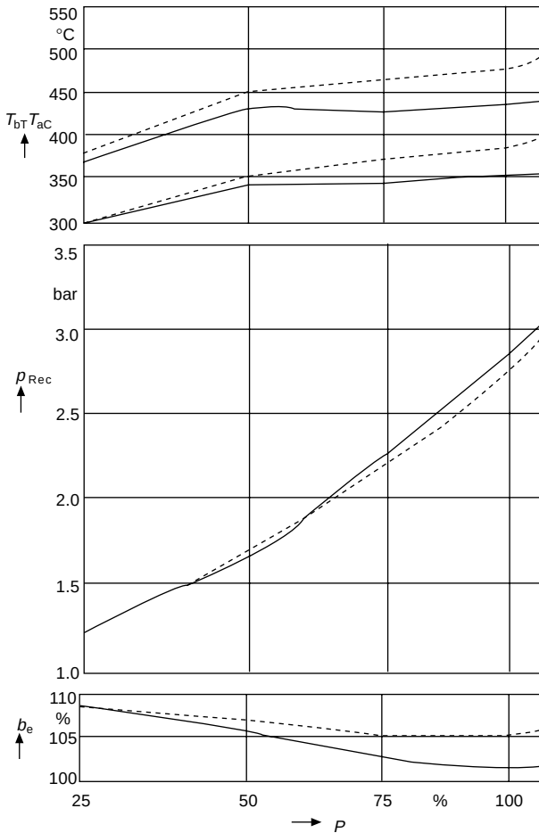
FIGURE 7.30 Turbocharger retrofit benefits exhaust-gas temperatures and specific fuel consumption of an ABB VTR..1 turbocharger exhibiting low efficiency (dashed lines) compared with a replacement VTR..4 turbocharger operating with a markedly higher efficiency (continuous lines)
