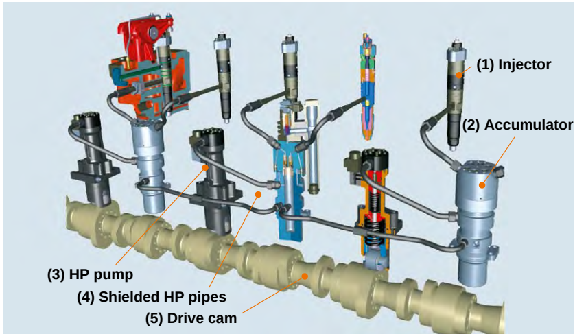
FIGURE 8.23 CR fuel system for Wärtsilä medium-speed engines
