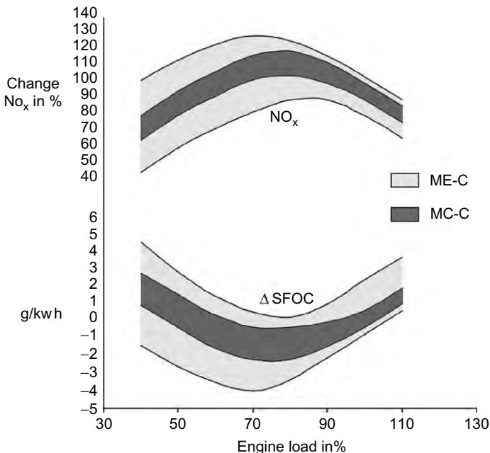
FIGURE 10.40 Flexibility of the electronically controlled ME concept compared with a traditional camshaft-controlled MC-C engine in terms of \text{NO}_x emissions and sfc
