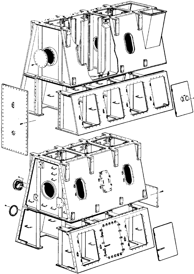
FIGURE 13.5 K-GF engine structural arrangement
