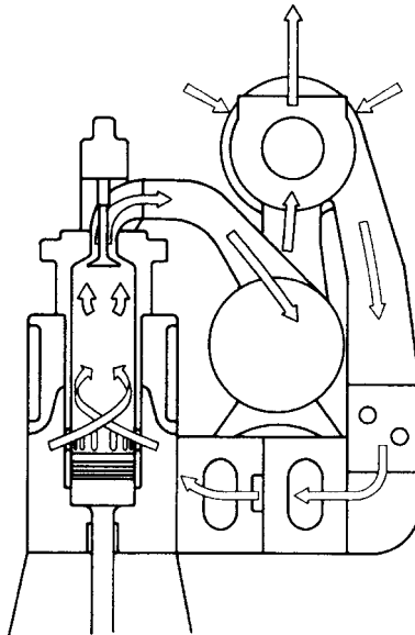
FIGURE 12.1 Uniflow scavenging system for RTA engine series
