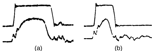
FIGURE 8.6 Fuel line pressure (lower line) and needle lift diagrams. (a) At high load. (b) At low load (Delphi Bryce)
