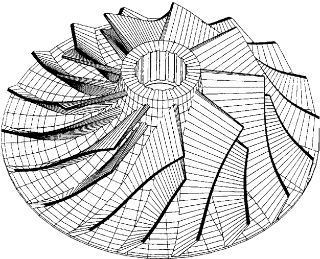
FIGURE 7.22 A 3D CAD visualization of the Napier 457 turbocharger impeller, showing the one-piece intervanned swept-back design with tip rake
