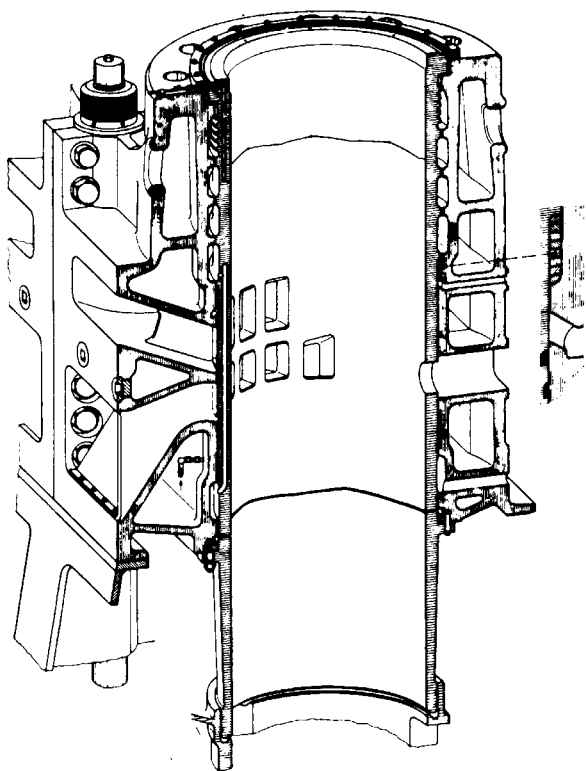
FIGURE 15.14 Cylinder liner and jacket
