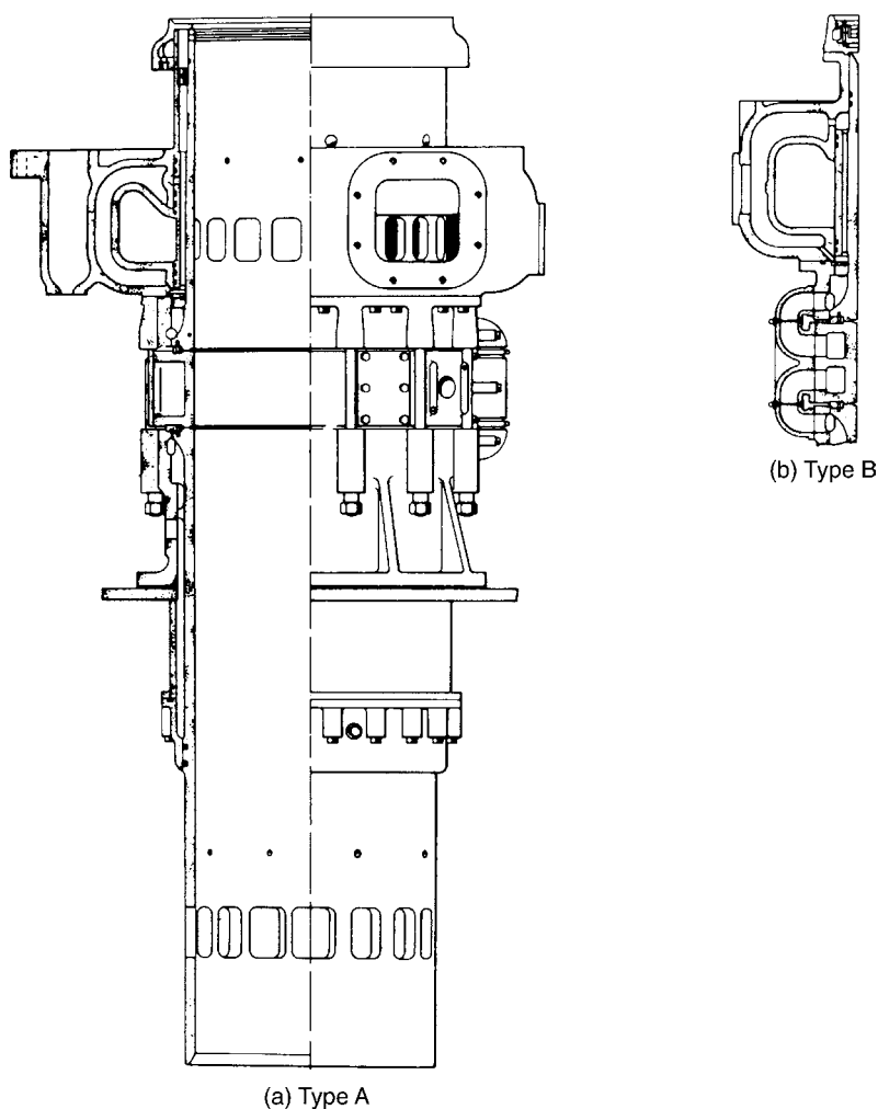
FIGURE 14.6 Cylinder assembly
