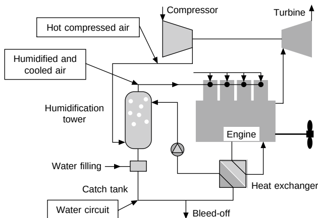
FIGURE 3.8 Schematic diagram of HAM system for NO x emission reduction
